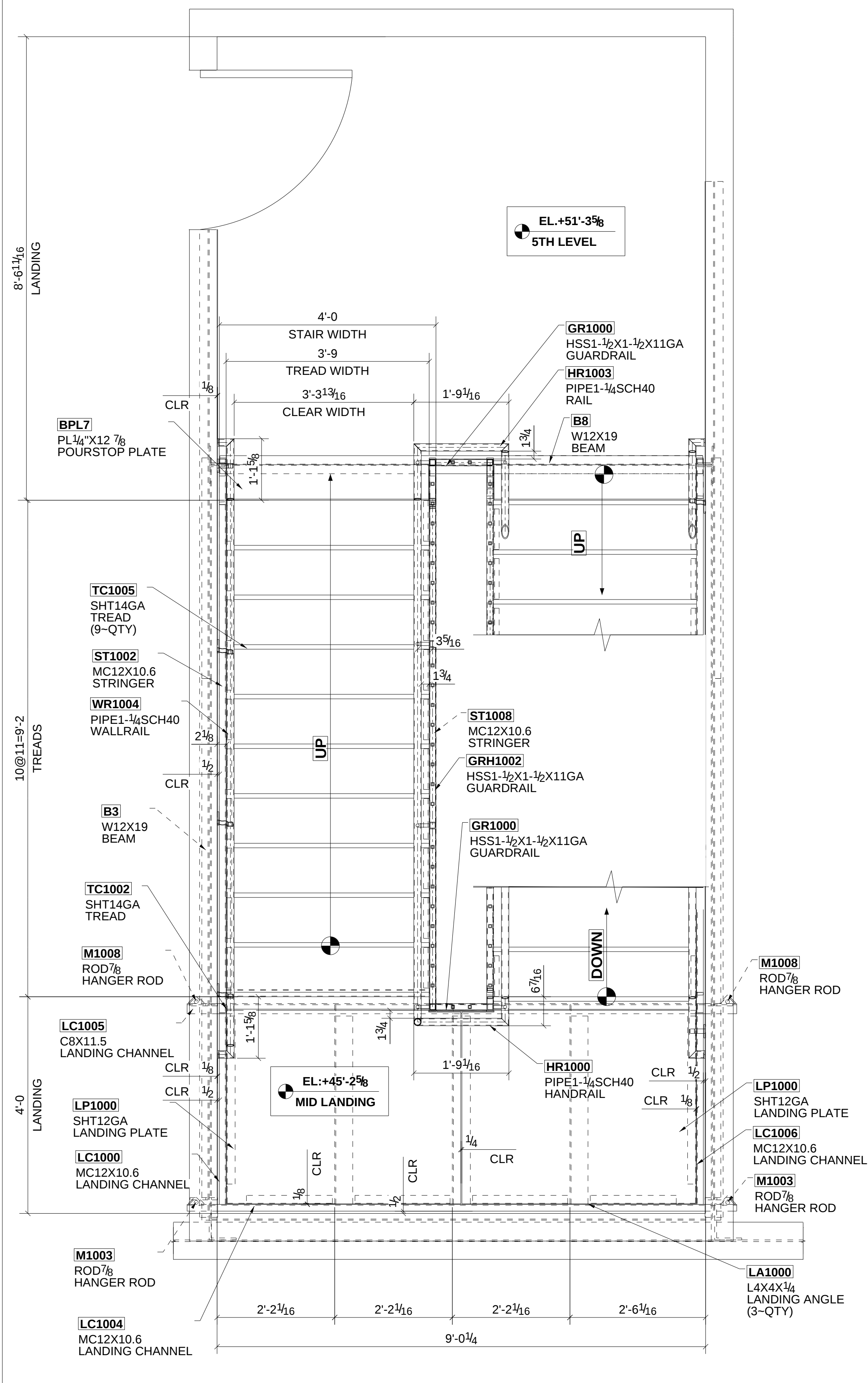
ENLARGED STAIR#1 PALN @ LEVEL 4 MID LANDING SCALE: 1:16
