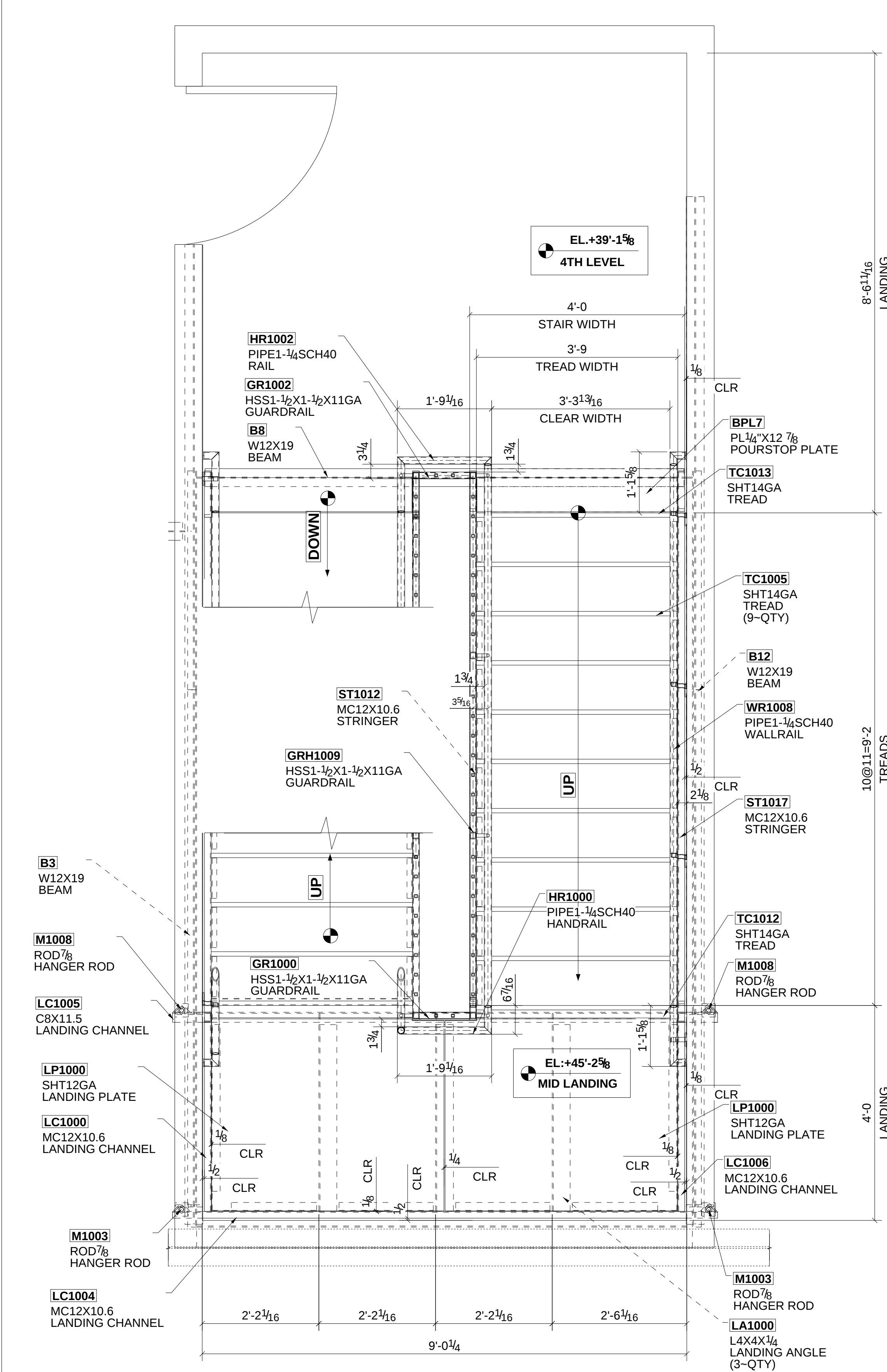
ENLARGED STAIR#1 PALN @ LEVEL4 SCALE: 1:16
