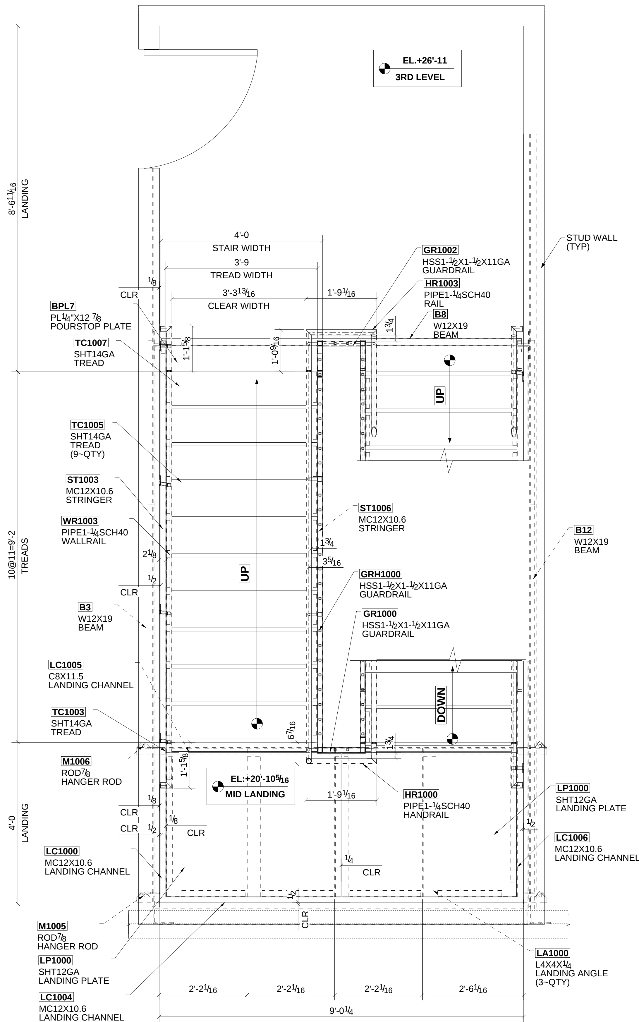
ENLARGED STAIR#1 PALN @ LEVEL 2 MID LANDING SCALE: 1:16
