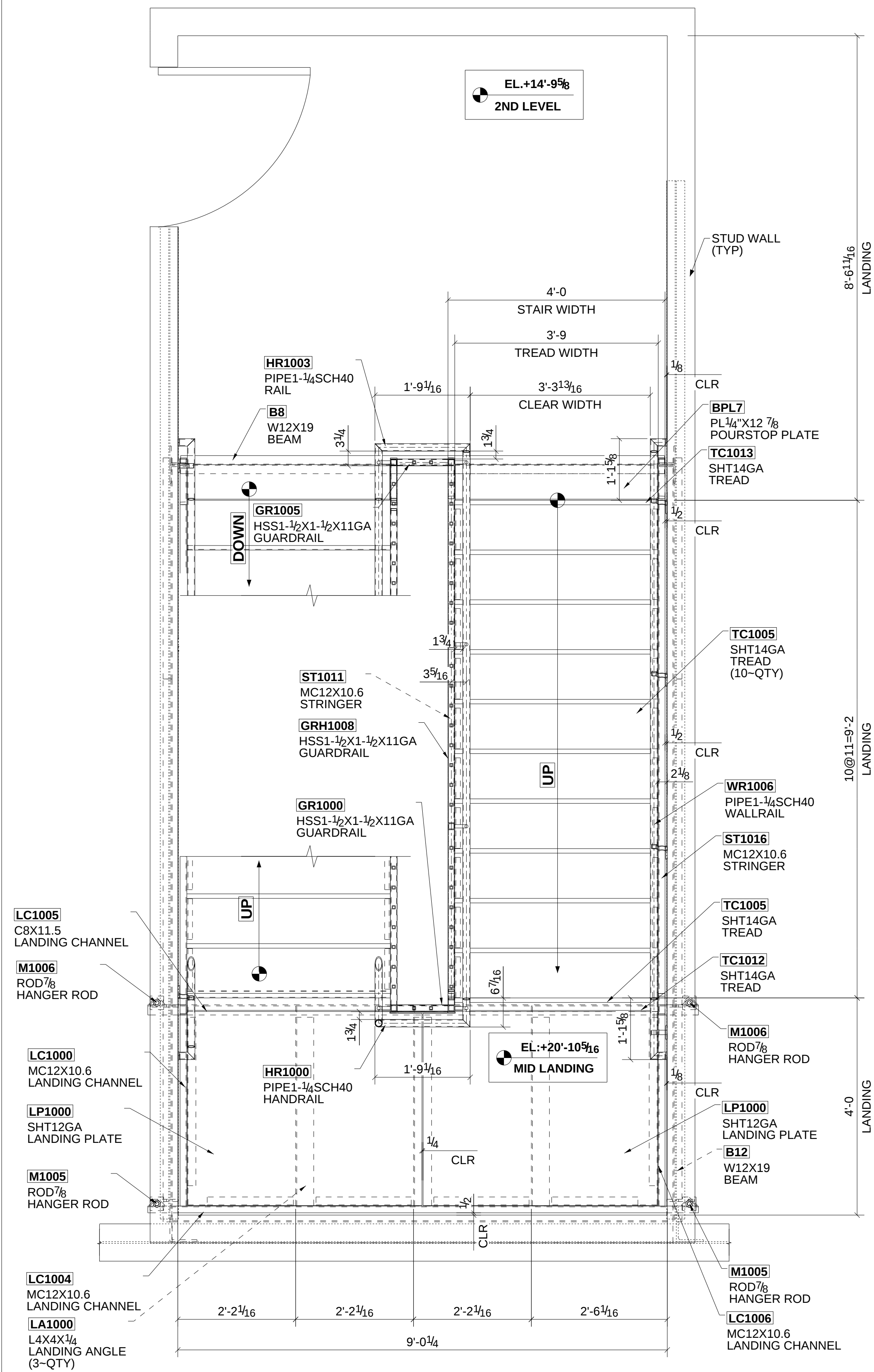
ENLARGED STAIR#1 PALN @ LEVEL 2 SCALE: 1:16
