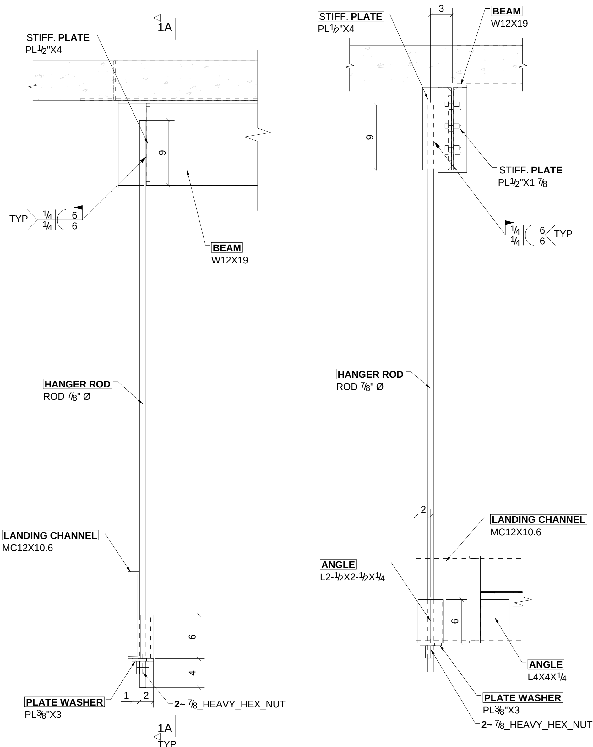
TYPICAL HANGER ROD DETAIL
