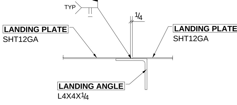
SECTION D - D
