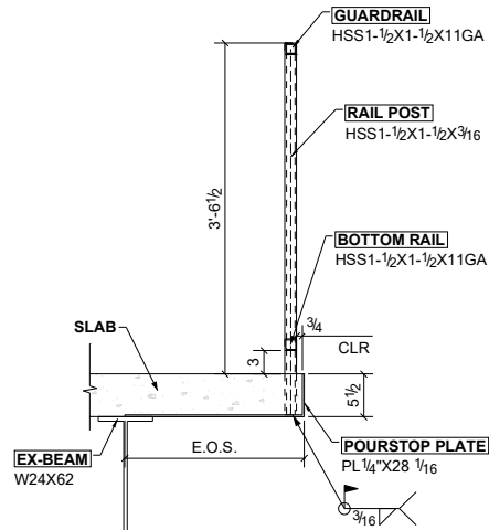
TYPICAL PLATFORM GUARDRAIL DETAIL SCALE: 1:12
