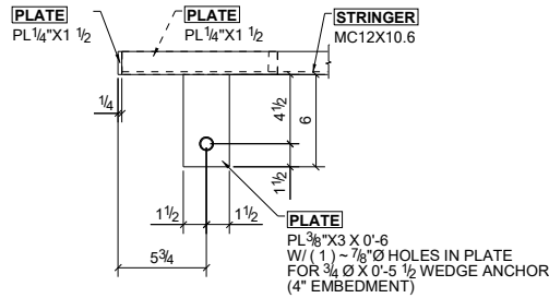
SECTION 1-1
