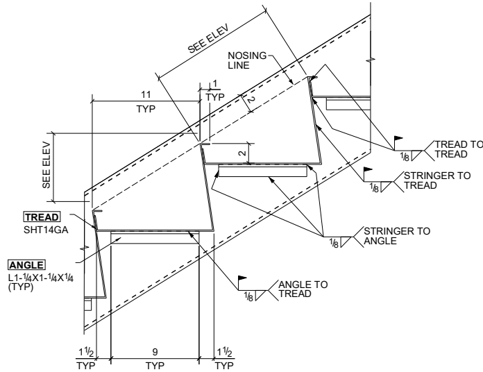
TYPICAL TREAD DETAIL SCALE: 1:6
