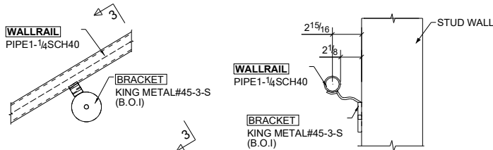
SECTION 3-3
