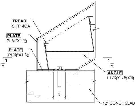
TYPICAL STRINGER BOTTOM TO SLAB DETAIL SCALE: 1:6
