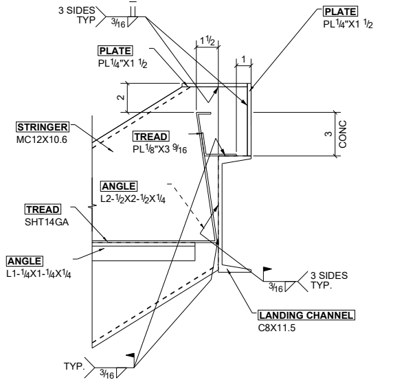
TYPICAL OUTER STRINGER TO HEADER CONNECTION. SCALE: 1:4
