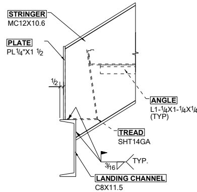
TYPICAL INNER STRINGER TO HEADER CONNECTION. SCALE: 1:6
