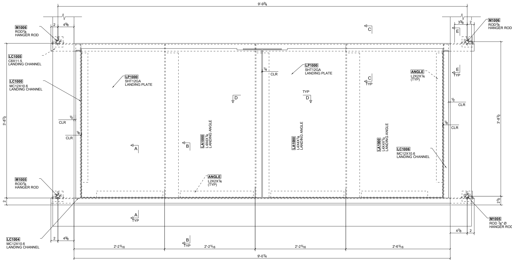
TYPICAL PLATFORM PLAN SCALE: 1:6
