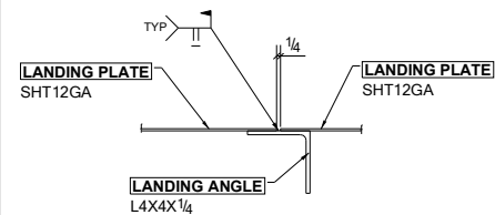
SECTION D - D
