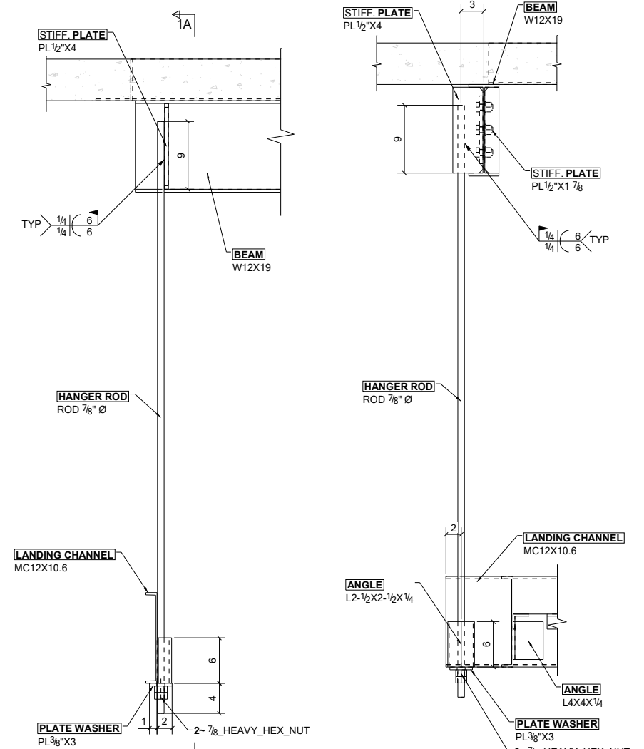
TYPICAL HANGER ROD DETAIL
