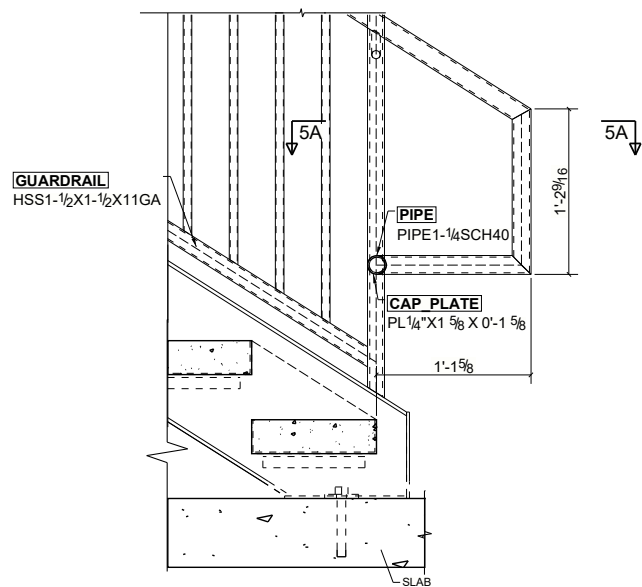
DETAIL-5 E10 TYPICAL HANDRAIL EXTENSION DETAIL
