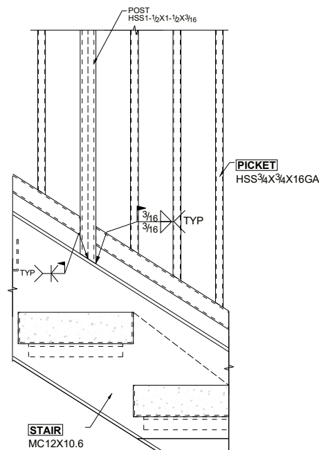
DETAIL-7 E10 TYPICAL STRINGER TO POST DETAIL
