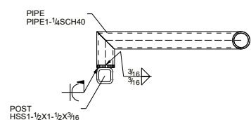
5A - 5A
