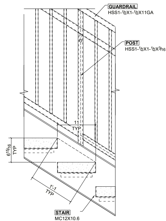
DETAIL-6 E10 TYPICAL OPEN RISERS DETAIL
