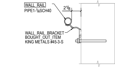
TYPICAL WALL BRACKET CONNECTION DETAIL E17
