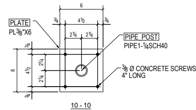
TYPICAL CANE RAIL BASE PLATE CONNECTION DETAIL
