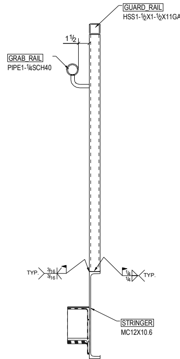
TYPICAL GUARD RAIL SECTION CONNECTION DETAIL
