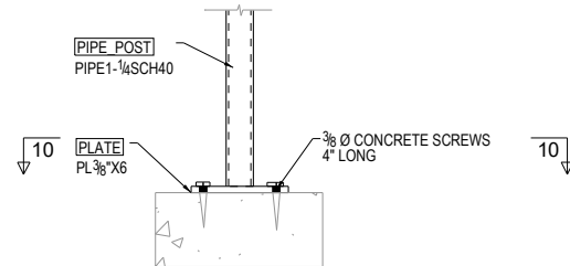
TYPICAL CANE RAIL BASE PLATE CONNECTION DETAIL
