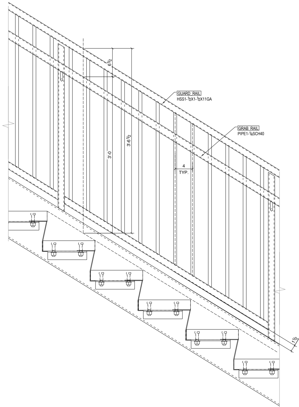
TYPICAL GUARD RAIL CONNECTION DETAIL E16
