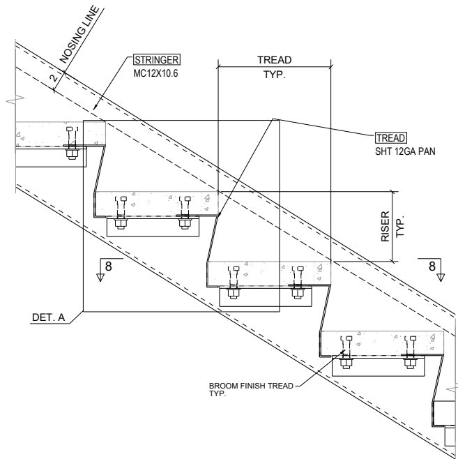
TYPICAL TREAD DETAIL
