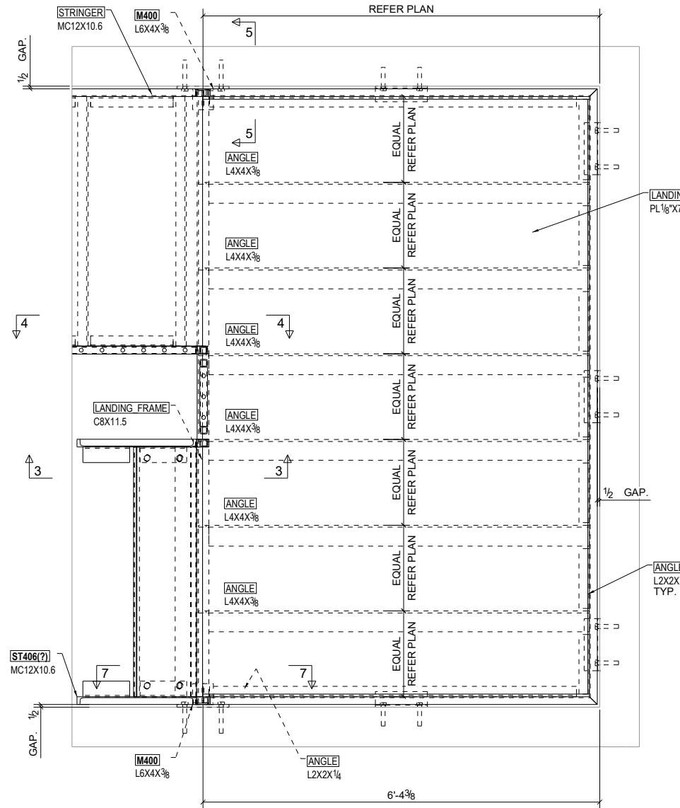
TYPICAL LANDING FRAMING DETAIL
