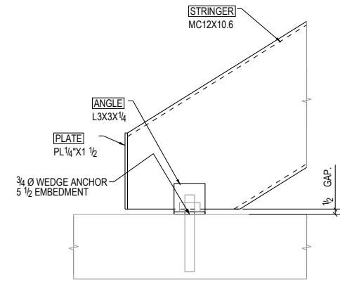
TYPICAL STAIR BASE DETAIL
