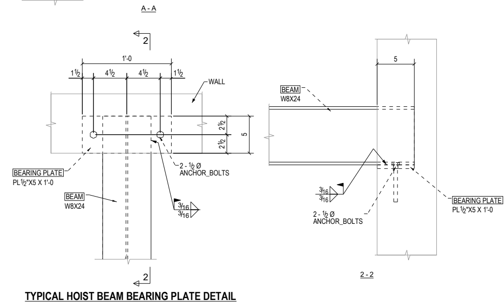
TYPICAL HOIST BEAM BEARING PLATE DETAIL
