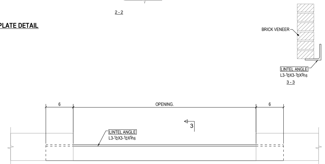
TYPICAL LINTEL DETAIL
