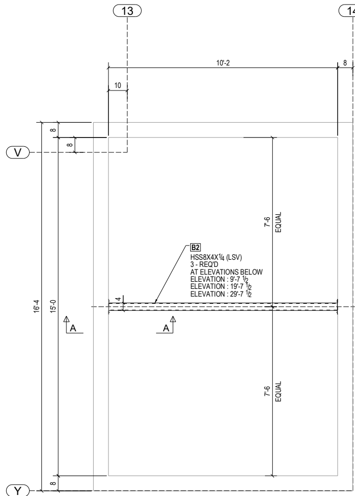
ELEVATOR DIVIDER BEAM PLAN REFER SHEET : S1.1,S2.1,S3.1 PLAN NORTH
