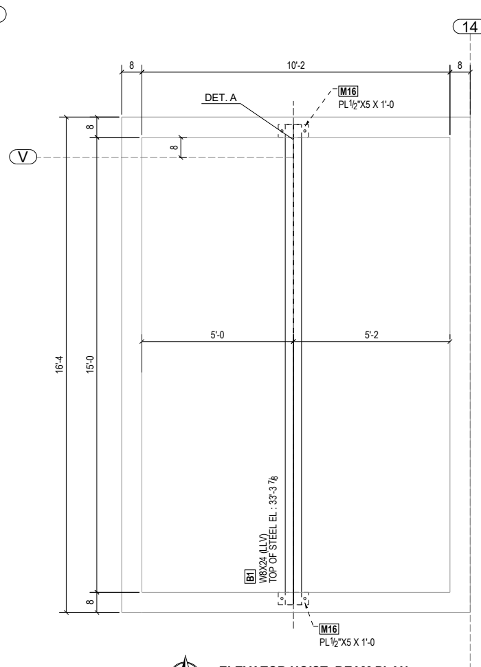
ELEVATOR HOIST BEAM PLAN REFER SHEET : S3.1,S10 PLAN NORTH
