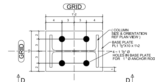
ANCHOR BOLT SETTING TYPE - 4 (REF.DWG.NO.: SB501) (AT 7 LOCATIONS)
