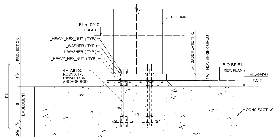
SECTION D - D (REF.DWG.NO.: SB501)
