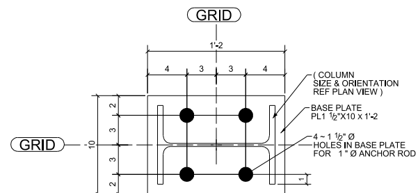
ANCHOR BOLT SETTING TYPE - 1 (REF.DWG.NO.: SB501) (AT 13 LOCATIONS)
