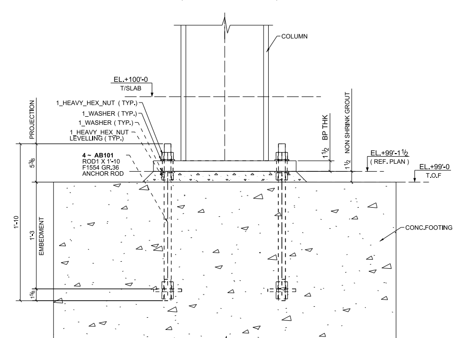
SECTION C - C (REF.DWG.NO.: SB501)
