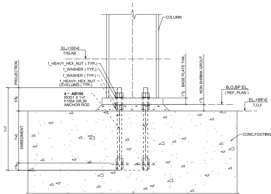
SECTION A - A (REF.DWG.NO.: SB501)
