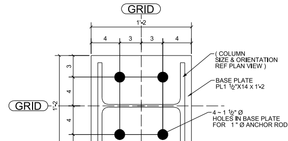
ANCHOR BOLT SETTING TYPE - 2 (REF.DWG.NO.: SB501) (AT 6 LOCATIONS)
