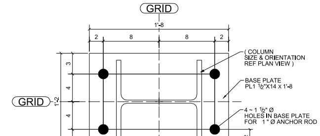
ANCHOR BOLT SETTING TYPE - 3 (REF.DWG.NO.: SB501) (AT 8 LOCATIONS)
