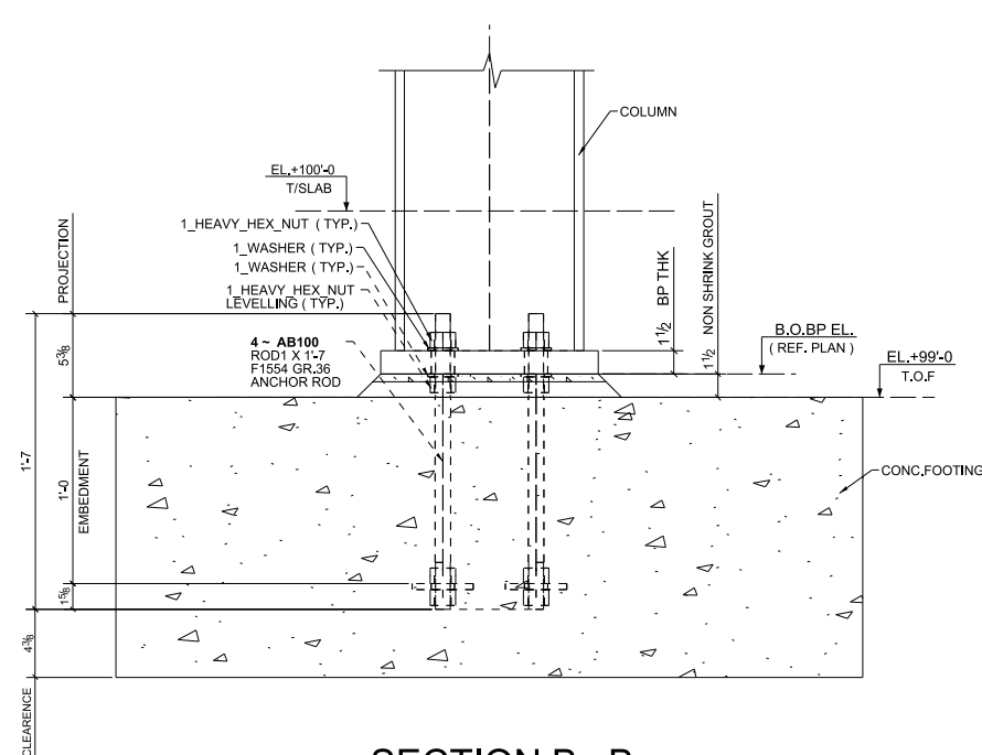
SECTION B - B (REF.DWG.NO.: SB501)
